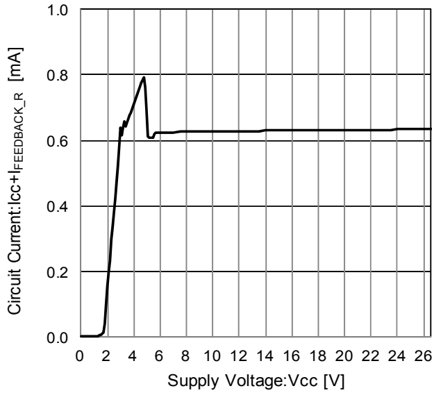
Figure 12. Circuit Current (I FEEDBACK_R (Note 1) \cong 75\mu\text{A} ) (Note 1) I FEEDBACK_R is the current through external Feed Back resistor.
