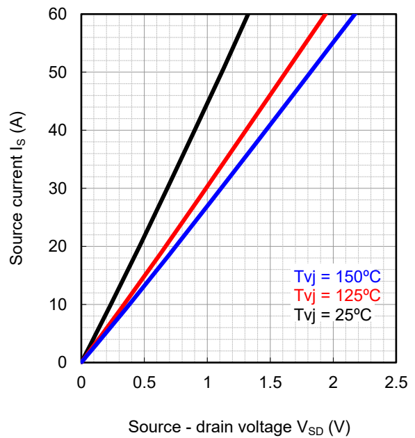
Figure 11. Forward characteristic of diode V_{GS} = 18V (Typ.)
