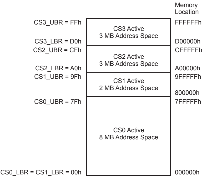
Figure 6. Example: Memory Chip Select
