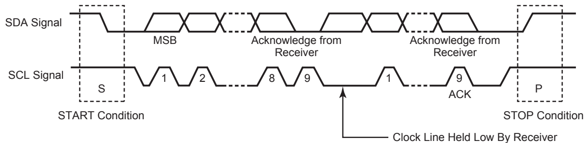
Figure 34. I²C Frame Structure
