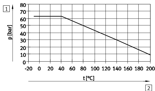
Fig. 5 Pressure-temperature diagram
