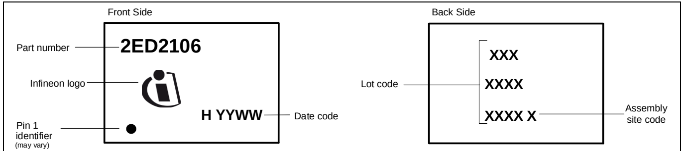
Figure 25 Marking information PG-DSO-8
