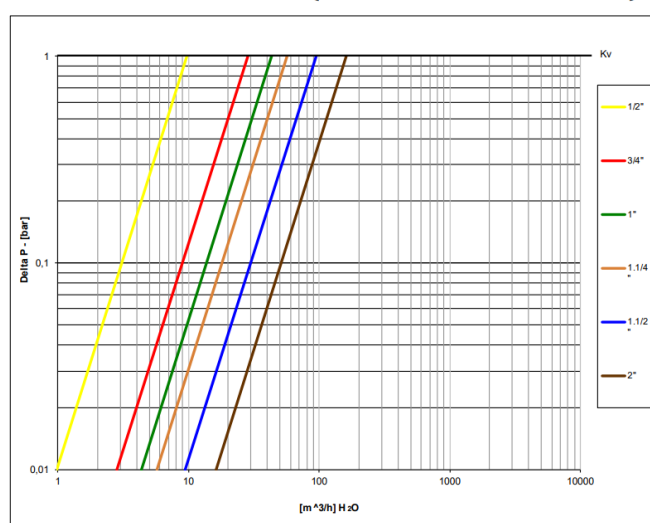
PRESSURE DROP CHART (STRAIGHT FLOW PATTERN)
