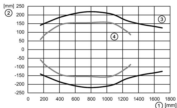
1: Distance; 2: Lobe acoustique; 3: Target 200 x 200 mm; 4: Cible Ø 25 mm
