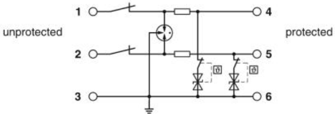
Circuit diagram
