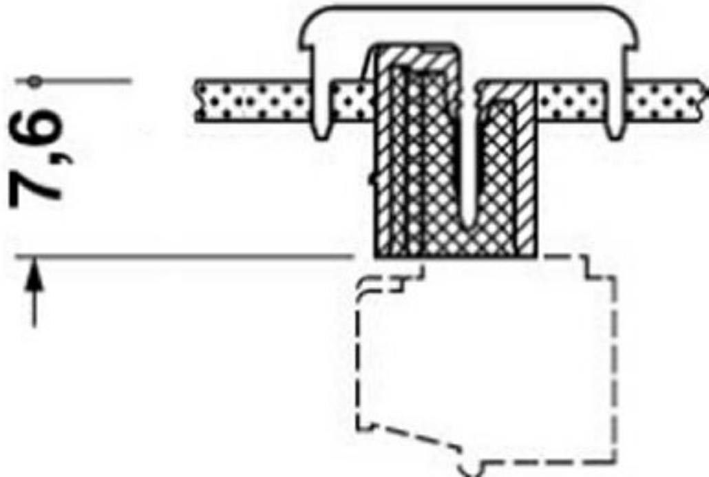
Dimensional drawing
