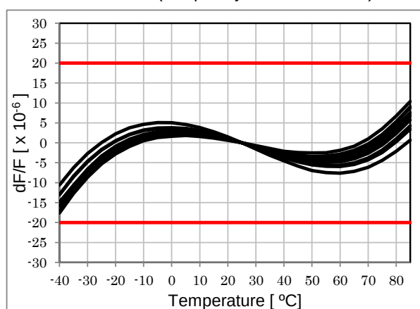
Frequency vs. Temperature characteristics (Frequency = 32 MHz, n=10)
