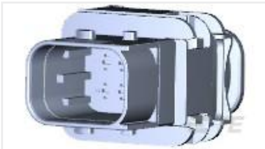
TE Part #1-1564512-1 8POS,TAB 1.6X0.6,TAB HSG,ASSY
