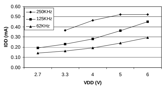
Figure 76. Typical I_{DD} in SLOW-WAIT vs. f_{CPU}
