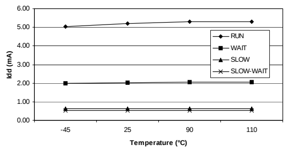
Figure 77. Typical I_{DD} vs. Temperature at V_{DD} = 5\text{V} and f_{CPU} = 8\text{MHz}
