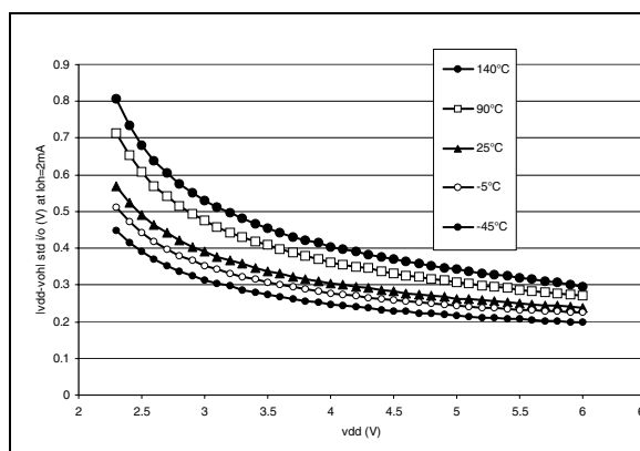
Figure 103. Typical V_{DD}-V_{OH} vs. V_{DD} (High Sink)
