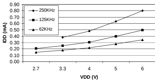
Figure 73. Typical I_{DD} in SLOW vs. f_{CPU}
