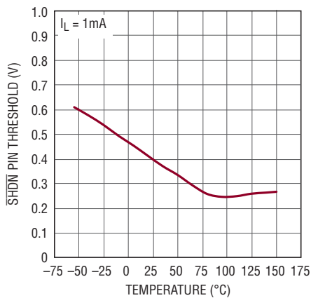
\overline{\text{SHDN1}} or \overline{\text{SHDN2}} Pin Threshold (On-to-Off)
