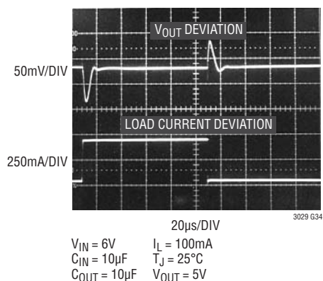
Transient Response, C_{BYP} = 0.01\mu\text{F}
