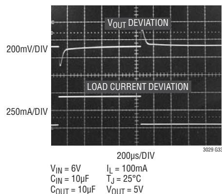
Transient Response, C_{BYP} = 0\text{pF}
