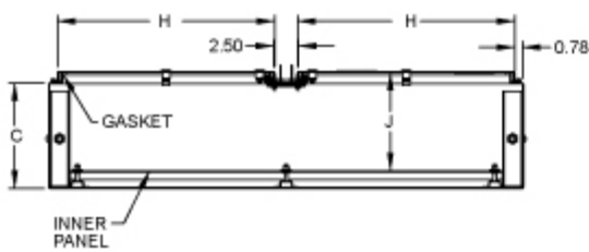
SECTION X-X
