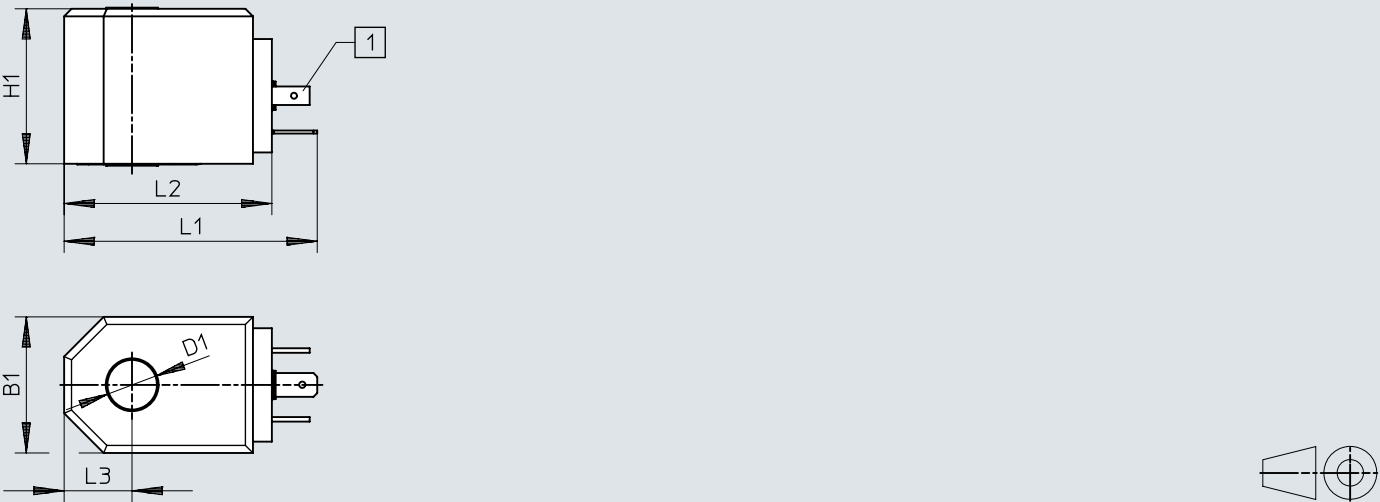
[1] Plug pattern type A, according to EN 175301-803
