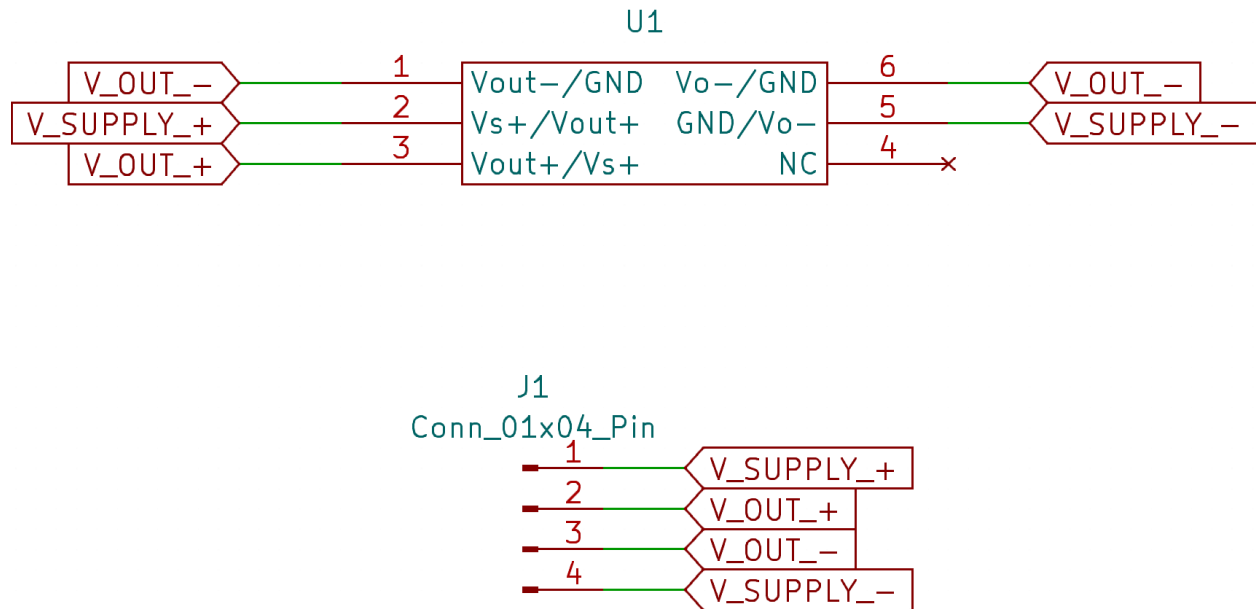
Figure 2. PSA070140-EB schematic.
