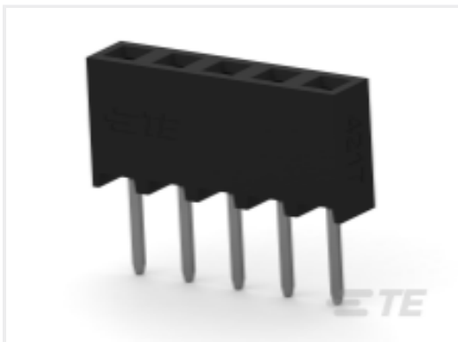
TE Part # 2307773-4 4P,2MM,BB,REC,SRVT,2.0,0.76AU,TR, W/CP
