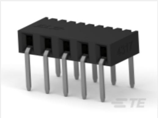
TE Part # 2307709-4 4P,2MM,B-B,REC,SRHZ,2.1,0.76AU,TR
