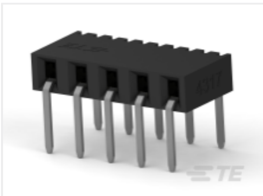
TE Part # 2307711-4 4P,2MM,B-B,REC,SRHZ,3.4,0.76AU, TUBE
