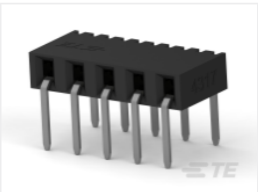
TE Part # 2307710-4 4P,2MM,B-B,REC,SRHZ,2.8,0.76AU,TB
