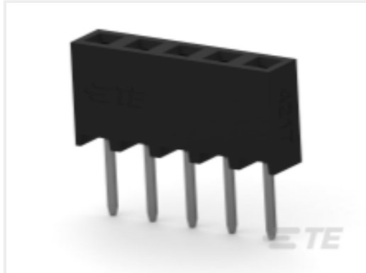
TE Part # 2314882-4 4P,2MM,BB,REC,SRVT,2.7,0.76AU,TB, W/CP
