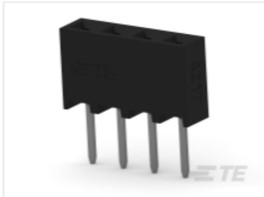
TE Part # 2314870-4 4P,2MM,BB,REC,SRVT,2.0,0.76AU,TB, W/CP
