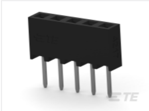
TE Part # 2307775-4 4P,2MM,B-B,REC,SRVT,3.2,0.76AU, TUBE
