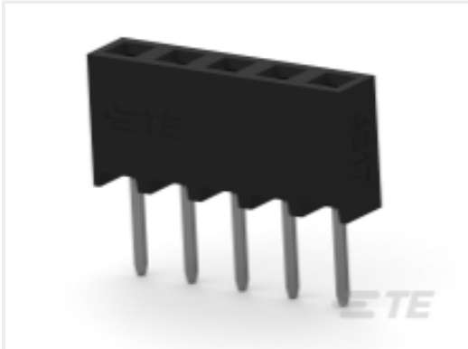
TE Part # 2307774-4 4P,2MM,BB,REC,SRVT,2.7,0.76AU,TR, W/CP
