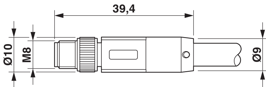
Dimensional drawing
