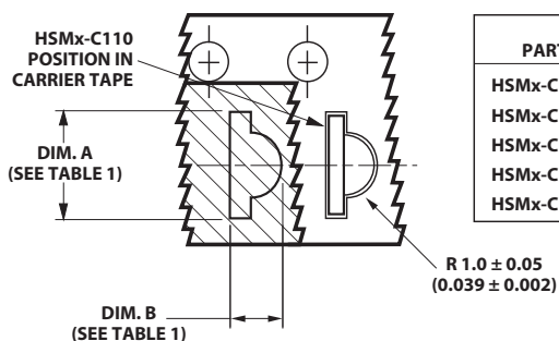
Figure 15. Tape dimensions.
