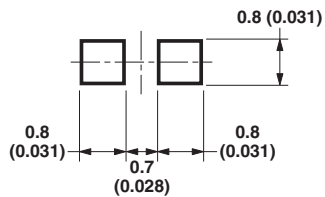
Figure 11. Recommended soldering pattern for HSMx-C190 and C191.
