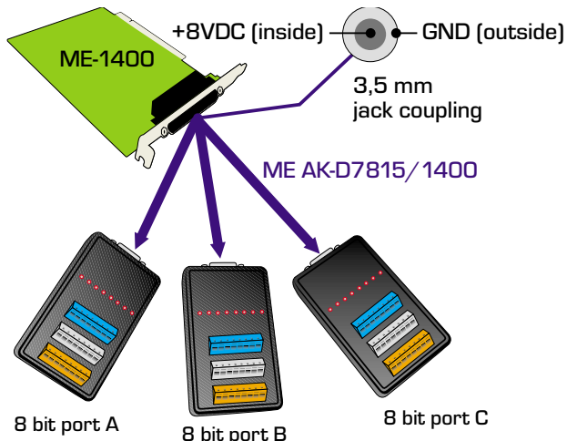
Diagram 3: Connection ME-1400/A/B
