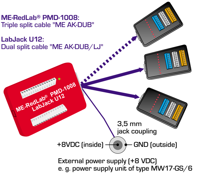
Diagram 2: Connection USB DAQ boxes
