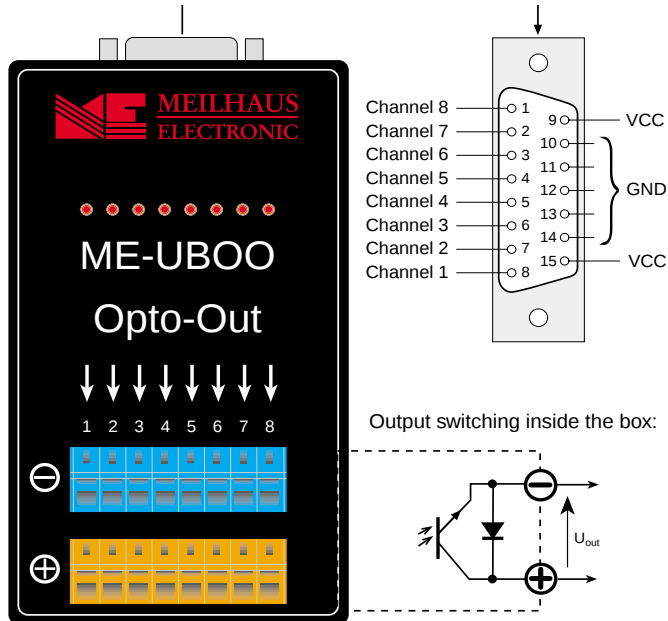
Diagram 1: Pinout
