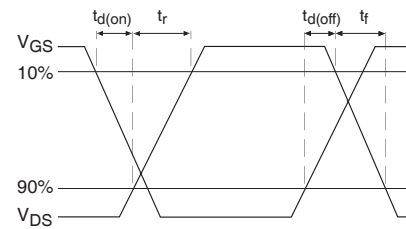
Fig 27b. Switching Time Waveforms
