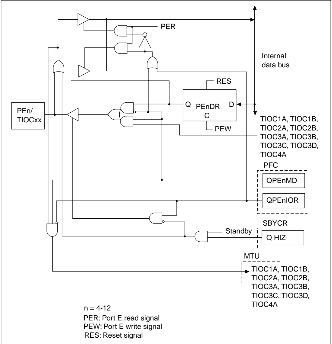
Figure B.36 PEEn/TIOcXX Block Diagram
