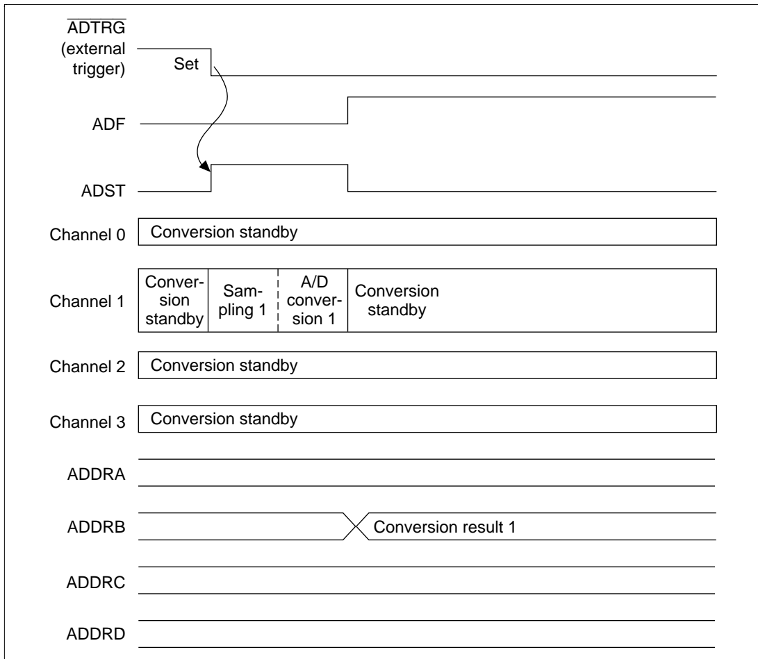
Figure 15.12 Conversion Start by ADTRG Conversion Start Trigger
