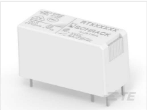
TE Part #8-1415898-6 RTSETA12
