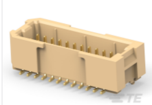
TE Part # 2484140-4 1.0mm P HPI 85deg 2x12 Pos
