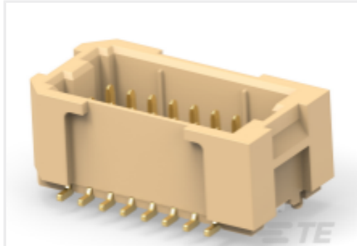
TE Part # 2484140-2 1.0mm P HPI 85deg 2x8 Pos
