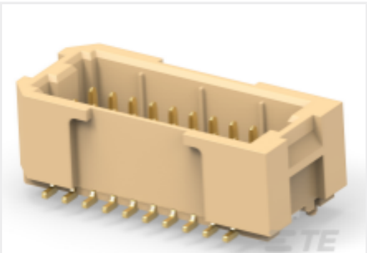
TE Part # 2484140-3 1.0mm P HPI 85deg 2x10 Pos
