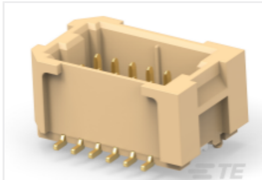
TE Part # 2484140-1 1.0mm P HPI 85deg 2x6 Pos
