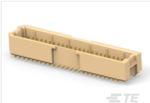
TE Part # 2484140-6 1.0mm P HPI 85deg 2x25 Pos
