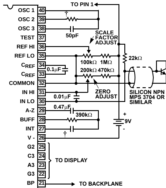
A silicon diode-connected transistor has a temperature coefficient of about -2\text{mV}/^{\circ}\text{C} . Calibration is achieved by placing the sensing transistor in ice water and adjusting the zeroing potentiometer for a 000.0 reading. The sensor should then be placed in boiling water and the scale-factor potentiometer adjusted for a 100.0 reading. † Value depends on clock frequency.
