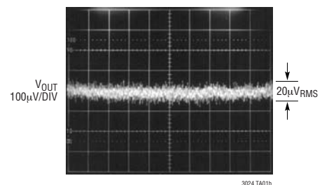
10Hz to 100kHz Output Noise
