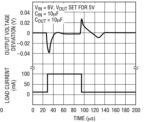
Output 2 Transient Response C_{BYP} = 0.01µF
