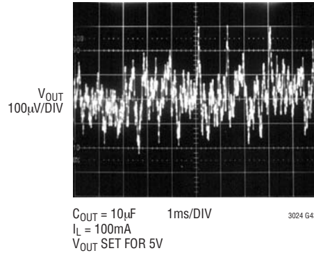
10Hz to 100kHz Output Noise C_{BYP} = 100pF
