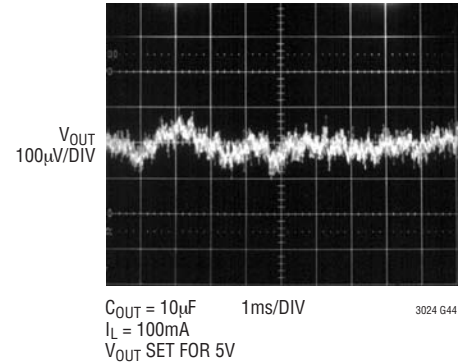
10Hz to 100kHz Output Noise C_{BYP} = 1000pF
