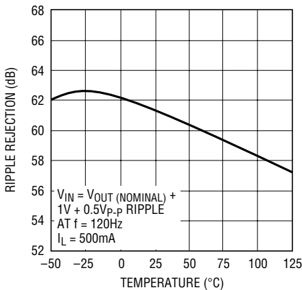
Output 1 Ripple Rejection
