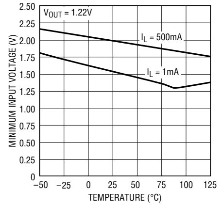
Output 1 Minimum Input Voltage
