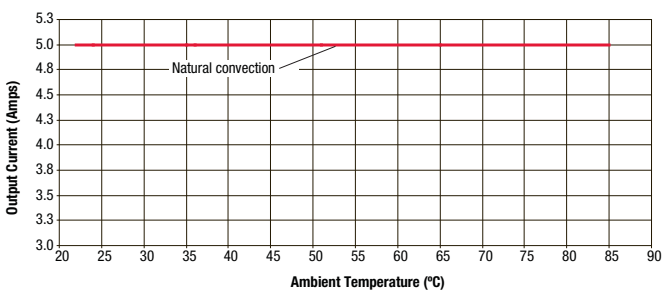
OKY-T/5-D12 Maximum Current Temperature Derating @ Sea Level (VIN = 12V, VOUT = 1V, airflow is transverse)
