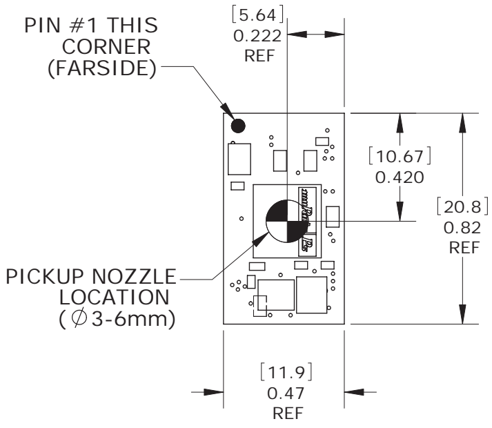
PICK & PLACE PICKUP (P/U)
