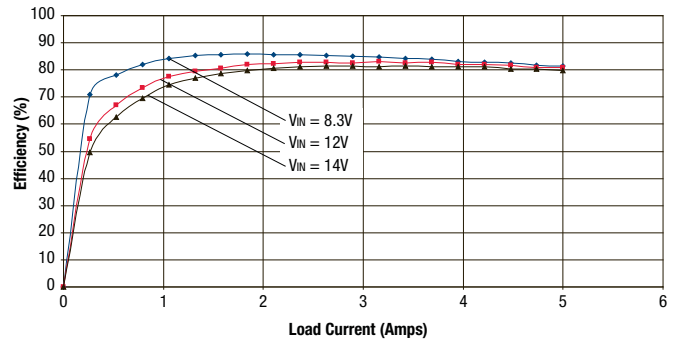
OKY-T/5-D12 Efficiency vs. Line Voltage and Load Current @ 25°C (Vout = 1V)
