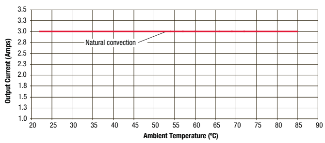
OKY-T/3-D12 Maximum Current Temperature Derating @ Sea Level (VIN = 12V, VOUT = .75V, airflow is transverse)
