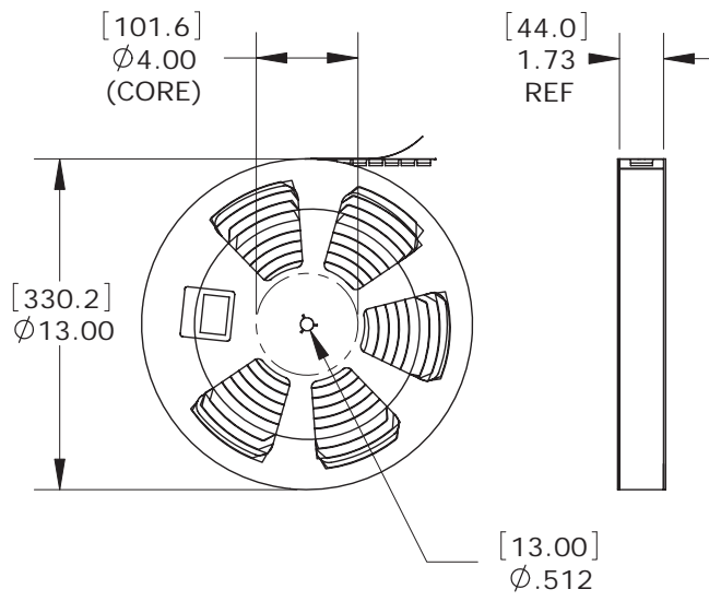
REEL INFORMATION (400 UNITS PER REEL)
