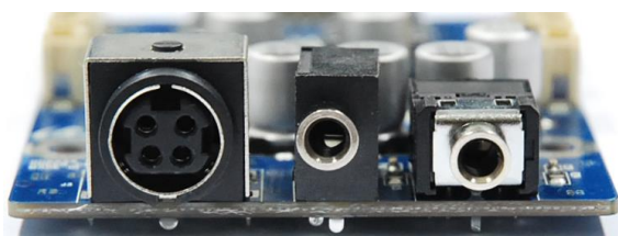
24V Ac/DC adaptor Type (connect with J3 barrel jack)
