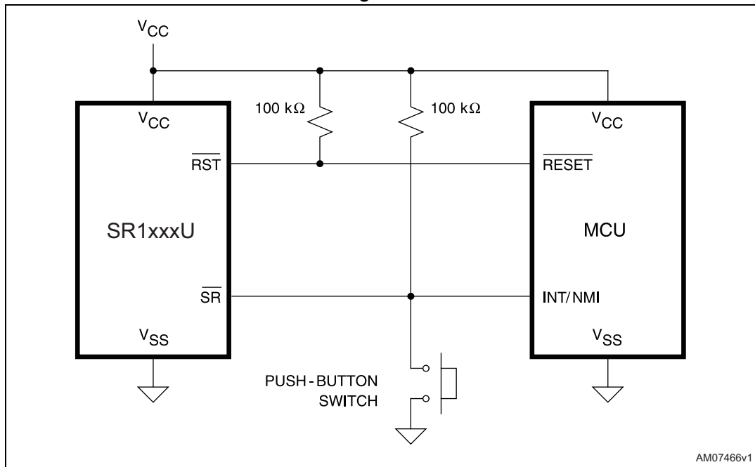
Figure 4. Typical application diagram - input, output and SR1xxxU device in one voltage domain
