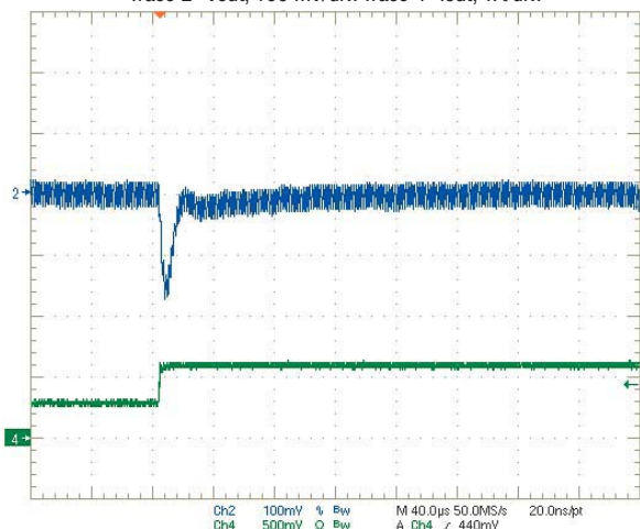
Step Load Transient Response (Vin=12V, Vout=2.5V, Load=0, Iout=1.5A to 3A) Trace 2=Vout, 100 mV/div. Trace 4=Iout, 1A/div.
