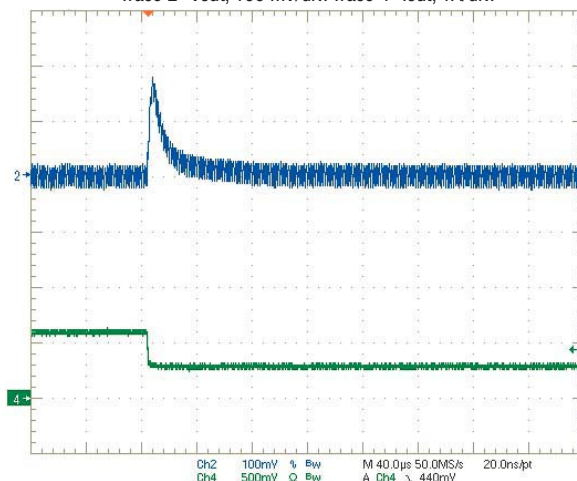
Step Load Transient Response (Vin=12V, Vout=2.5V, Load=0, Iout=3A to 1.5A) Trace 2=Vout, 100 mV/div. Trace 4=Iout, 1A/div.
