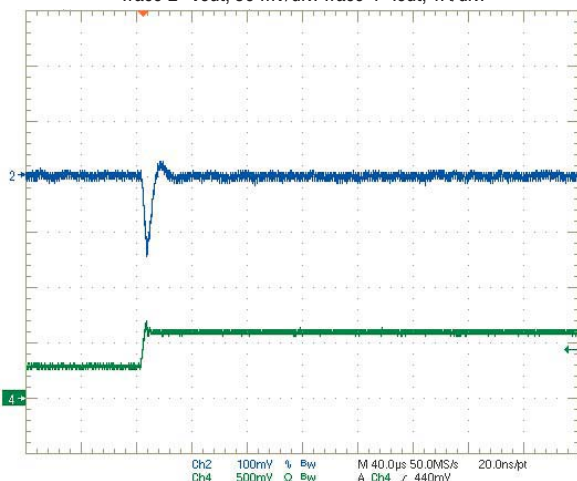
Step Load Transient Response (Vin=12V, Vout=0.591V, Cloud=0, Iout=1.5A to 3A) Trace 2=Vout, 50 mV/div. Trace 4=Iout, 1A/div.
