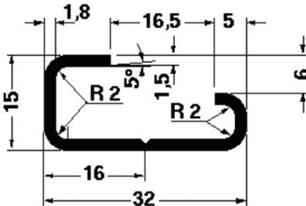
Dimensioned drawing
