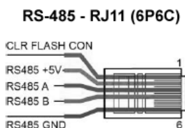
Fig.4. Pin assignment of the RJ11 connector - RS-485 Modbus
