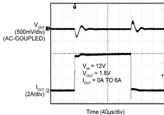
Transient Response
