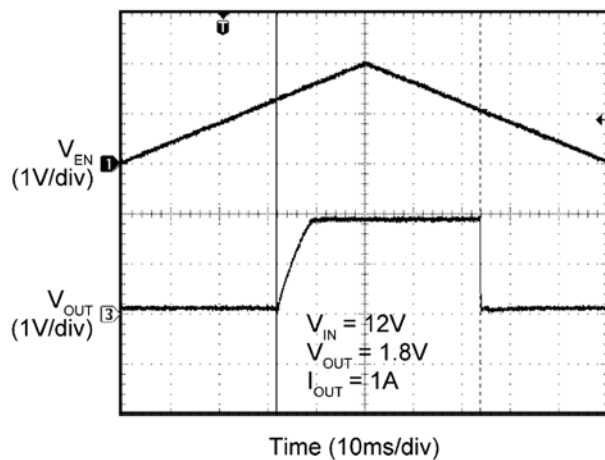
Enable Thresholds
