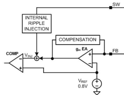
Figure 9. Internal Ripple Injection
