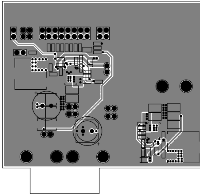
Figure 14. MIC24051 Evaluation Board Mid-Layer 2
