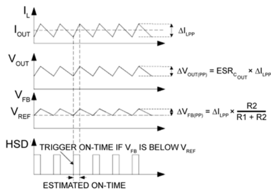
Figure 2. MIC24051 Control Loop Timing
