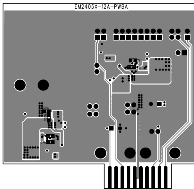
Figure 15. MIC24051 Evaluation Board Bottom Layer
