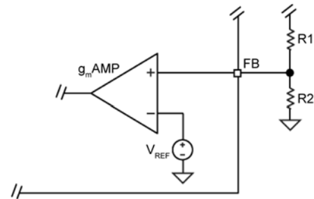
Figure 8. Voltage-Divider Configuration
