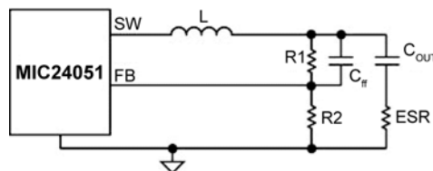
Figure 6. Inadequate Ripple at FB
