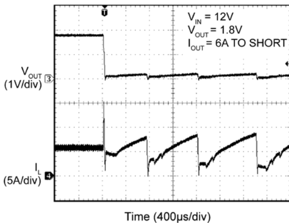
Short Circuit
