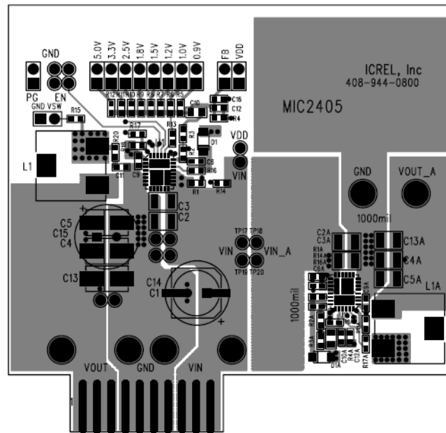
Figure 12. MIC24051 Evaluation Board Top Layer
