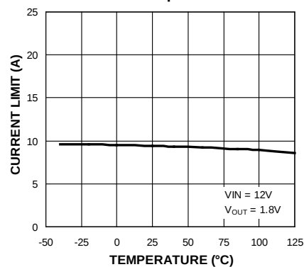
Output Current Limit vs. Temperature
