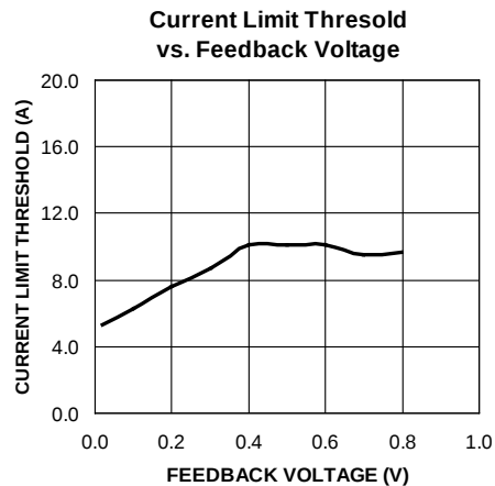
Figure 4. MIC24051 Current-Limit Foldback Characteristic
