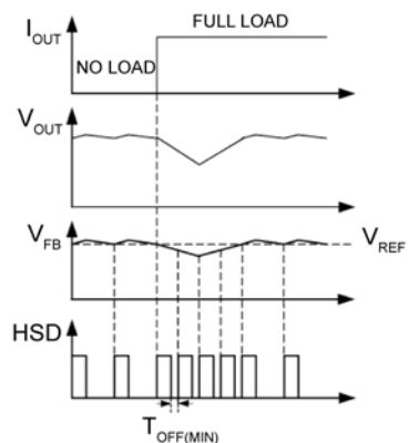
Figure 3. MIC24051 Load Transient Response
