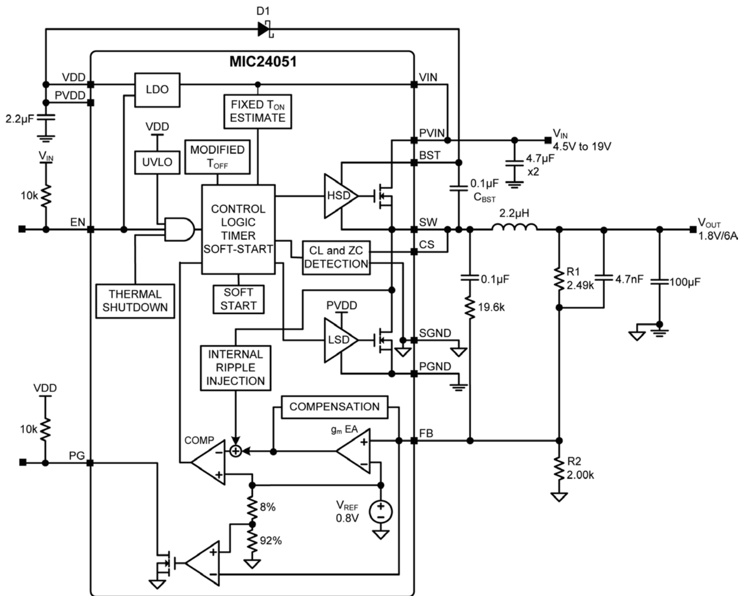
Figure 1. MIC24051 Block Diagram
