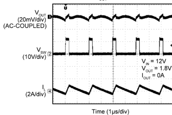
Switching Waveforms
