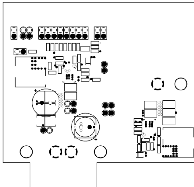
Figure 13. MIC24051 Evaluation Board Mid-Layer 1 (Ground Plane)
