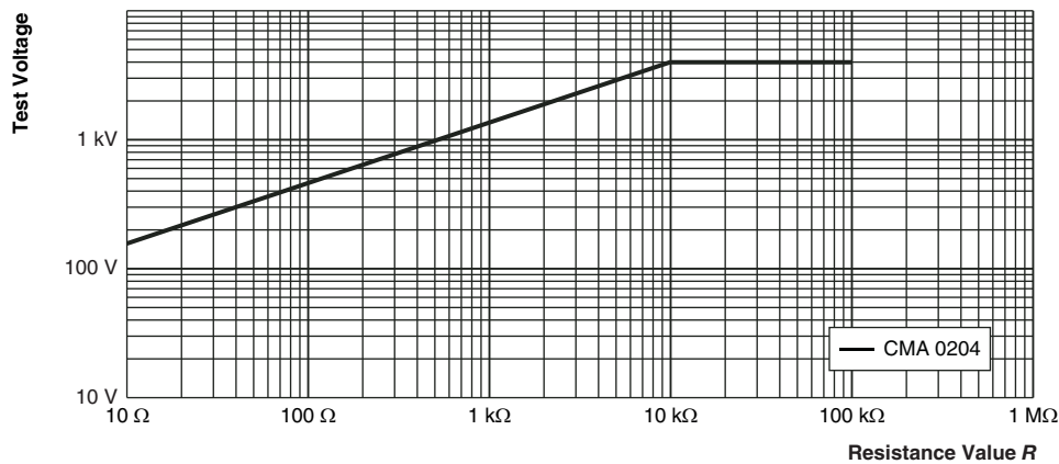
Fig. 6 - Source pulse capability of carbon film MINI-MELF resistors CMA 0204
