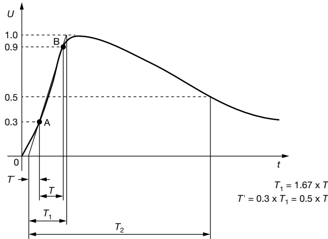
Fig. 5 - 1.2/50 \mu s or 10/700 \mu s single high voltage pulse
