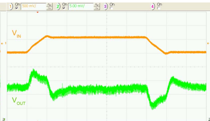
Figure 21. Line Transient 3.3V_{IN} to 3.9V_{IN} , 250mA Load, 10\mu s/div.
