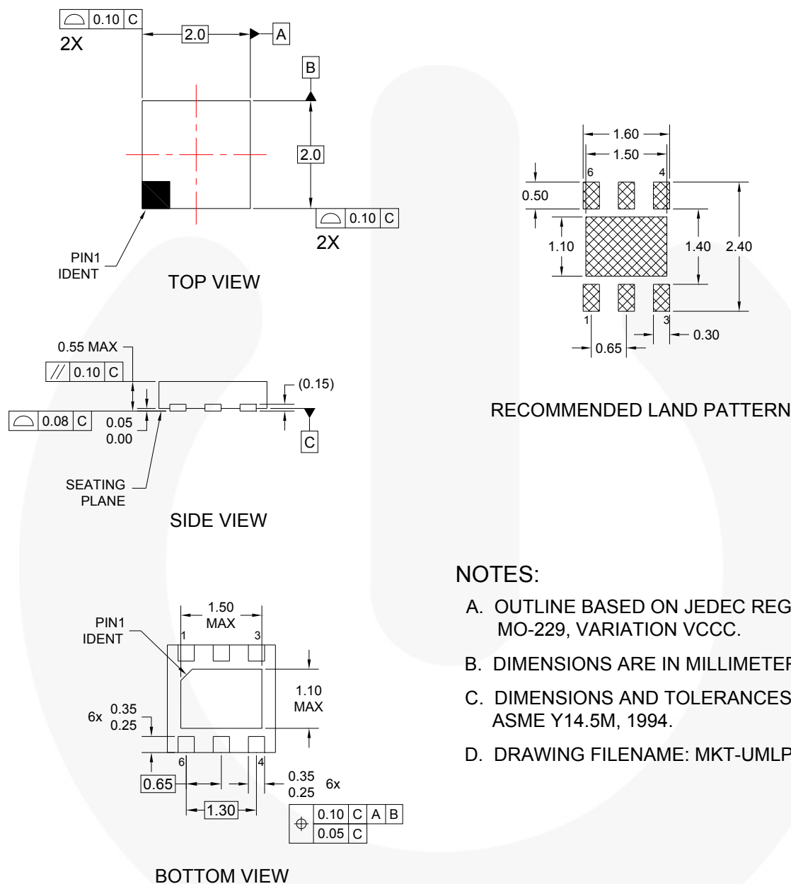
Figure 43. 6-Lead, 2 x 2mm, Ultra-Thin Molded Leadless Package (UMLP)
