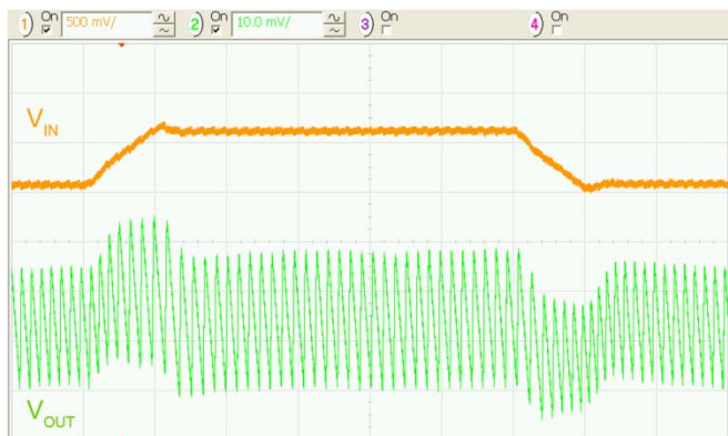
Figure 20. Line Transient 3.3V_{IN} to 3.9V_{IN} , 50mA Load, 10\mu s/div.
