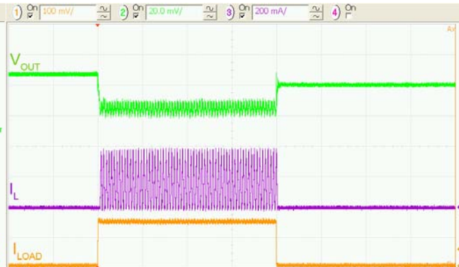
Figure 27. Load Transient 0 to 150mA, 3.6V_{IN}
