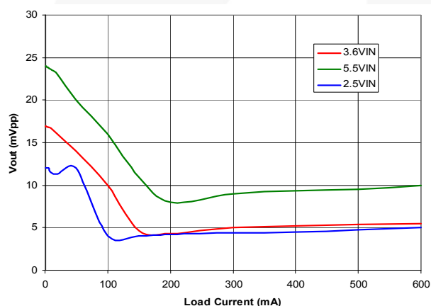
Figure 13. 1.233V OUT Peak-to-Peak Output Voltage Ripple
