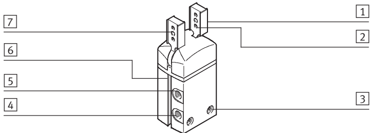
Fig. 1: Control sections and connections
