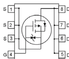
PG-DSO-8
