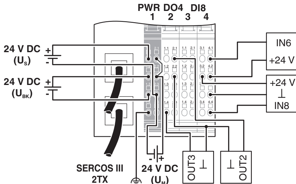
Connection diagram
