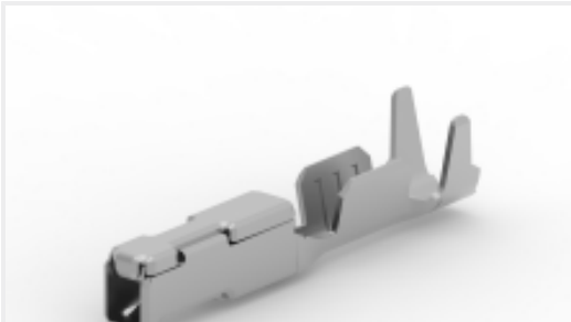
TE Part #2035334-8 CONTACT, FEMALE0.64 ,20.35SQMM
