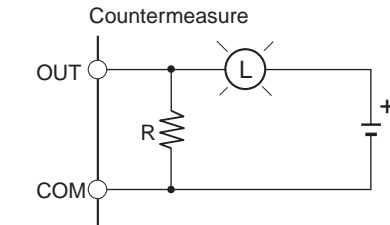
Providing about 1/3rd of the rated current to an incandescent light bulb.
