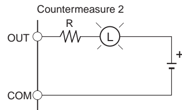
Using a limiting resistor
