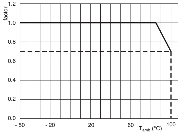
Max. DC and AC voltage as function of temperature
