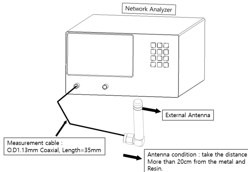
Figure 1 - VSWR Test
