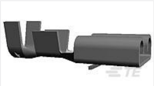
TE Part #60838-1 FF 250 REC 22-18AWG TPBR LP
