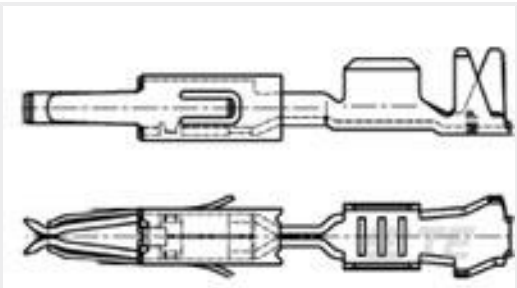
TE Part #969005-2 MT2 A REC 1.6 Contact SWS Sn
