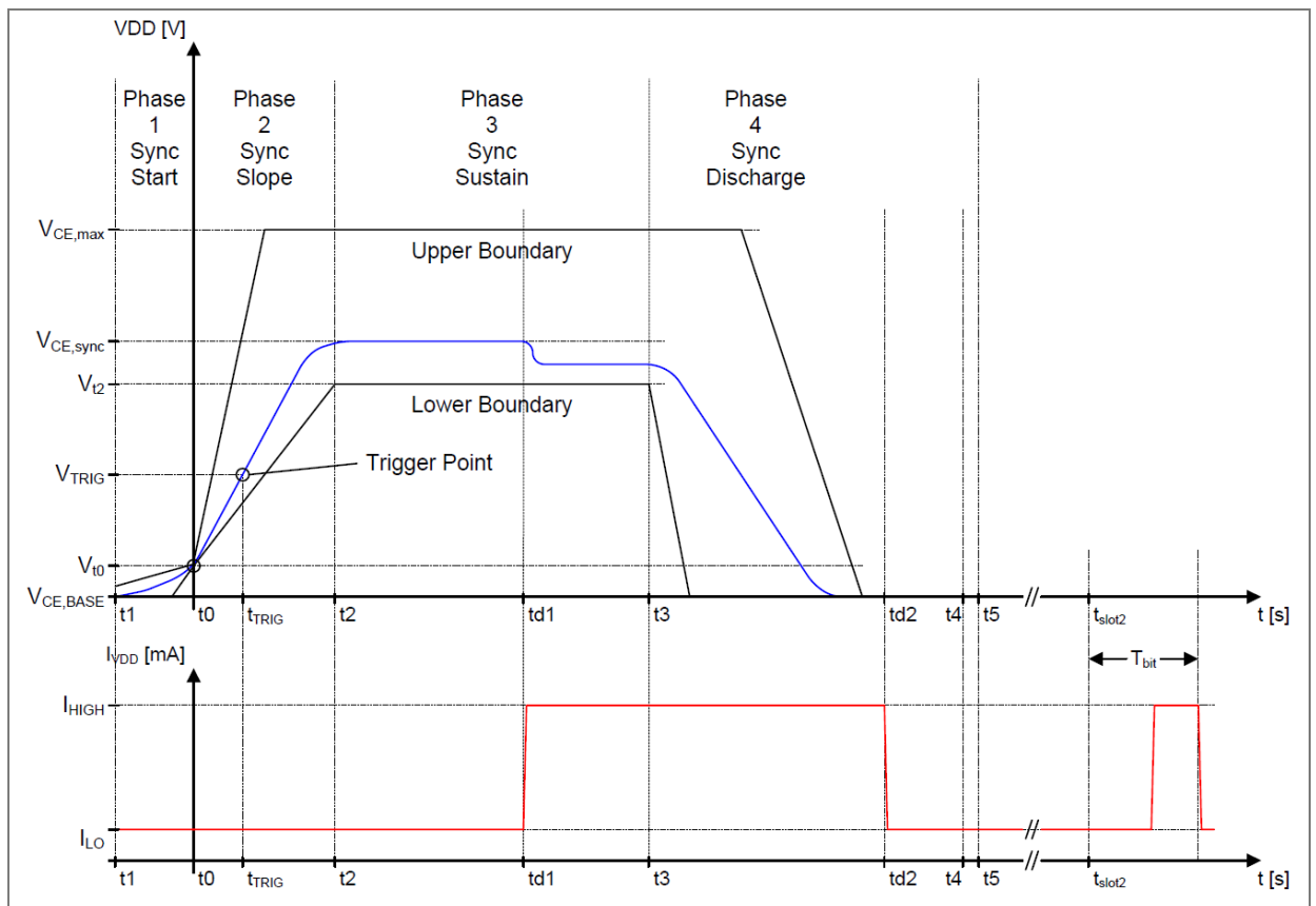
Figure 6: Synchronization signal from ECU with discharge by the AS5173
