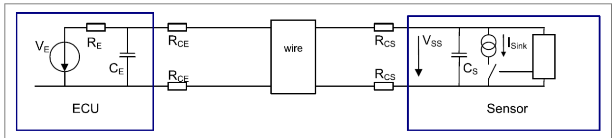
Figure 32: Asynchronous single sensor configuration
