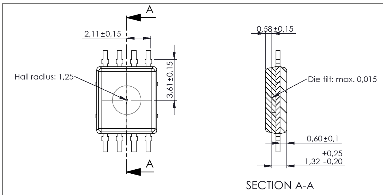
Figure 38: SIP die placement and hall array position
