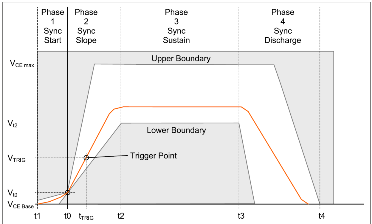
Figure 4: Synchronization signal
