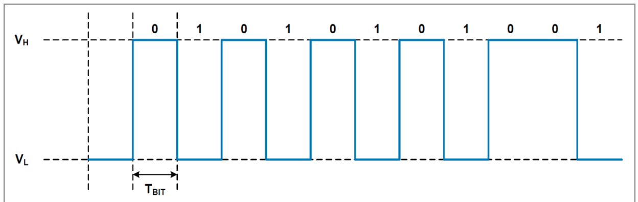
Figure 7: Bit encoding of programmer-to-sensor communication
