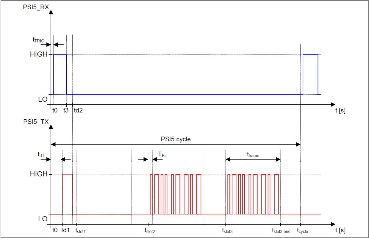
Figure 26: Synchronous mode P10P-500/3L with discharge pulse
