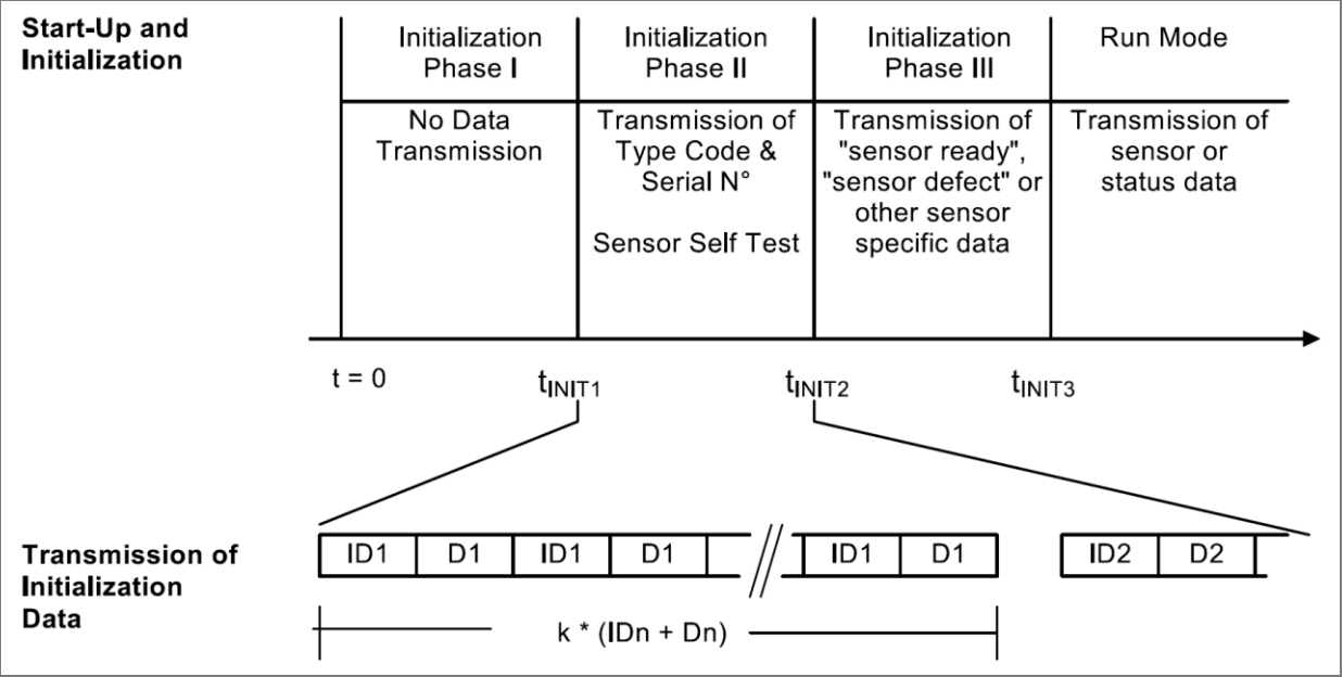
Figure 29: Start-up and initialization
