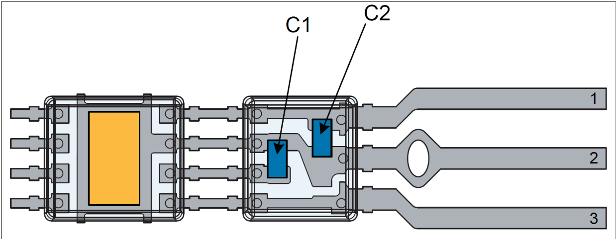
Figure 35: AS5173 components
