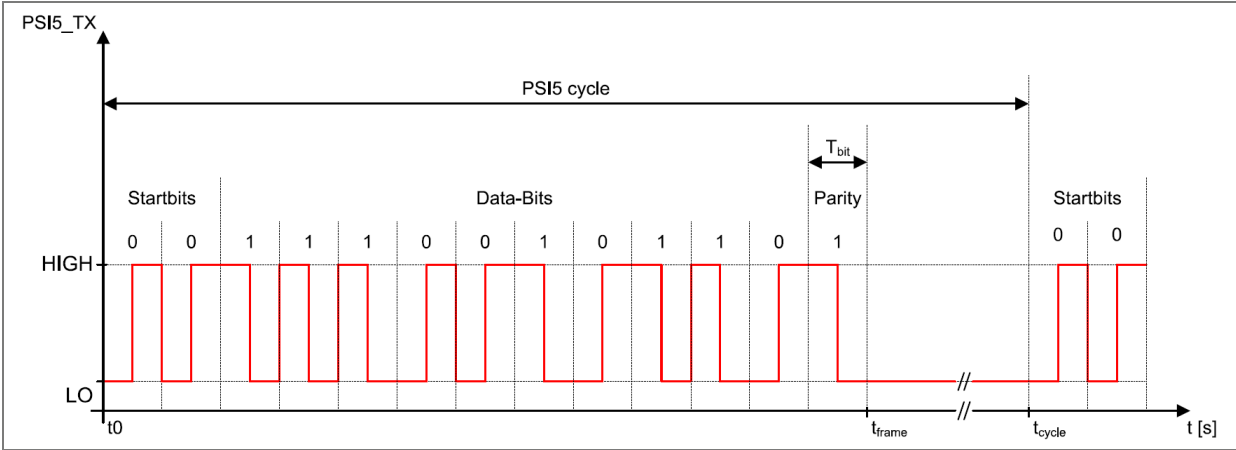
Figure 27: Asynchronous modes A10P- 50/1L and A10P-500/1L
