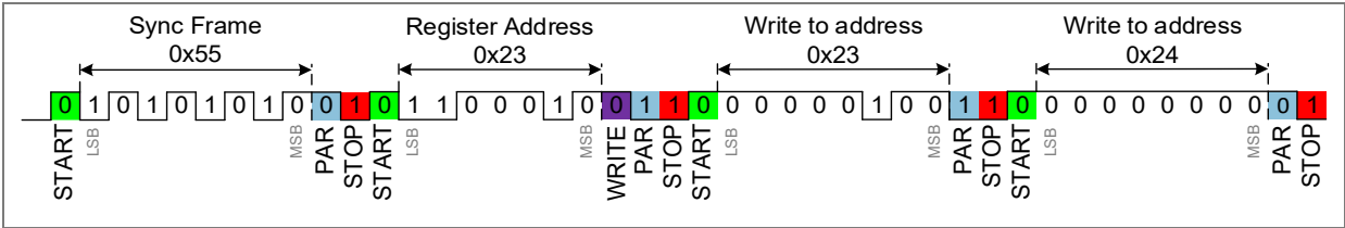
Figure 10: Example of WRITE (Reg[0x23] = 0x20 and Reg [0x24] = 0x00)
