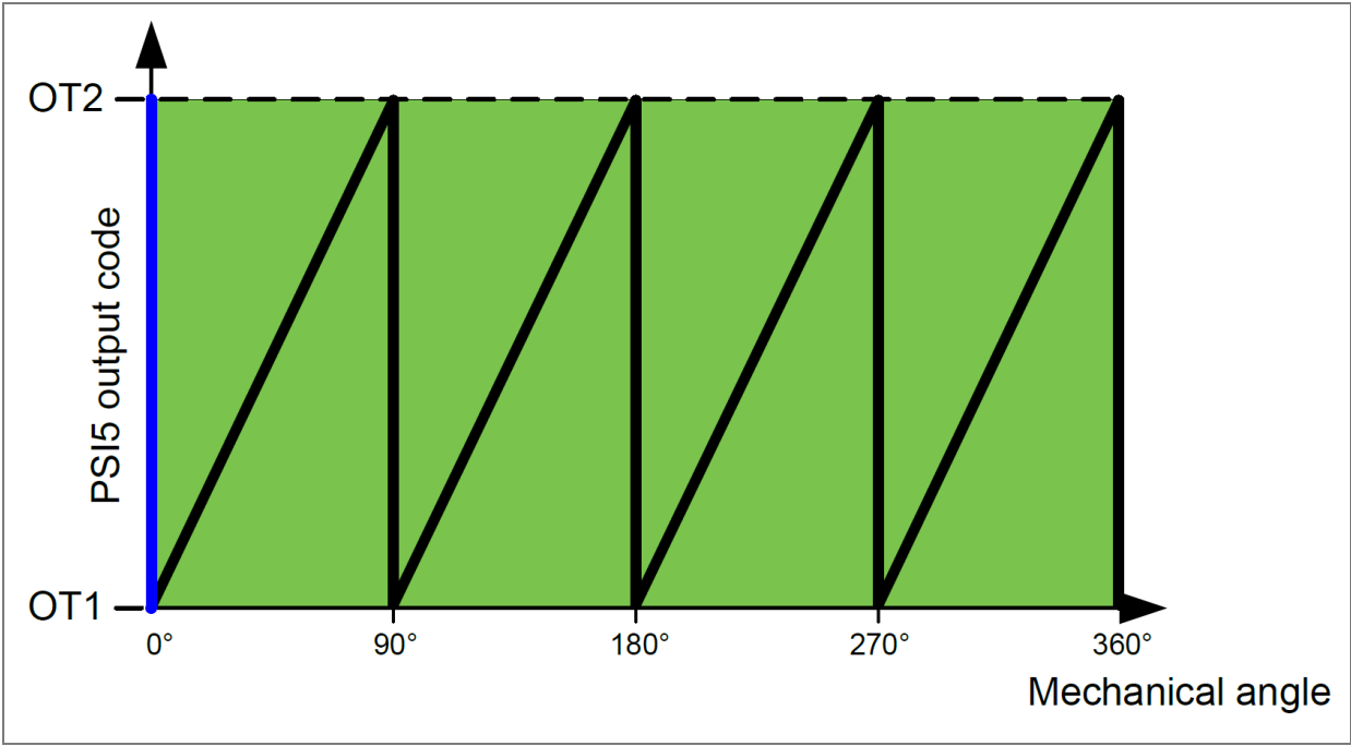
Figure 16: Quadruple quadrant
