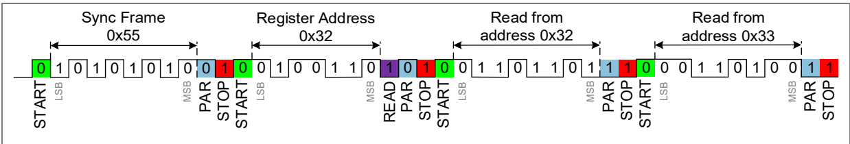
Figure 11: Example of READ (Reg[0x32] = 0xB6 and Reg [0x33] = 0x2C)
