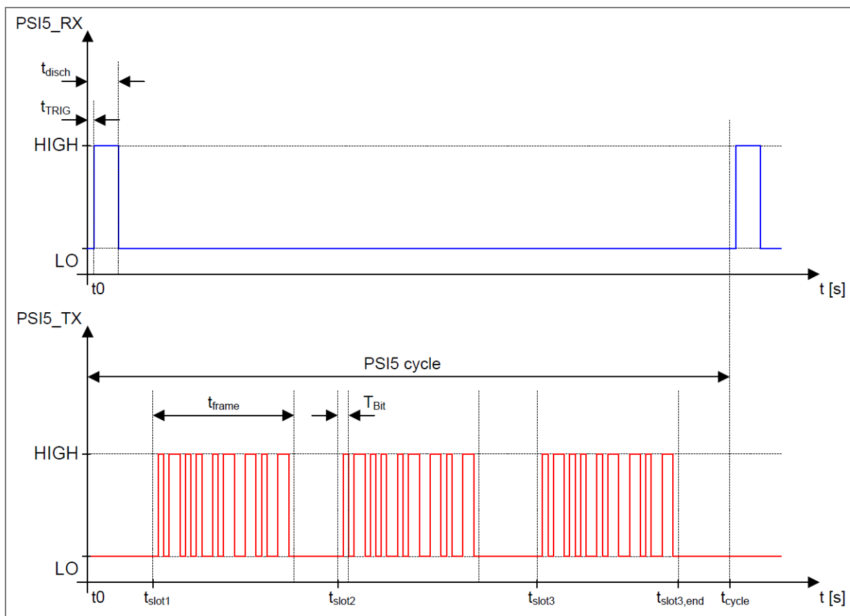
Figure 25: Synchronous mode P10P-500/3L
