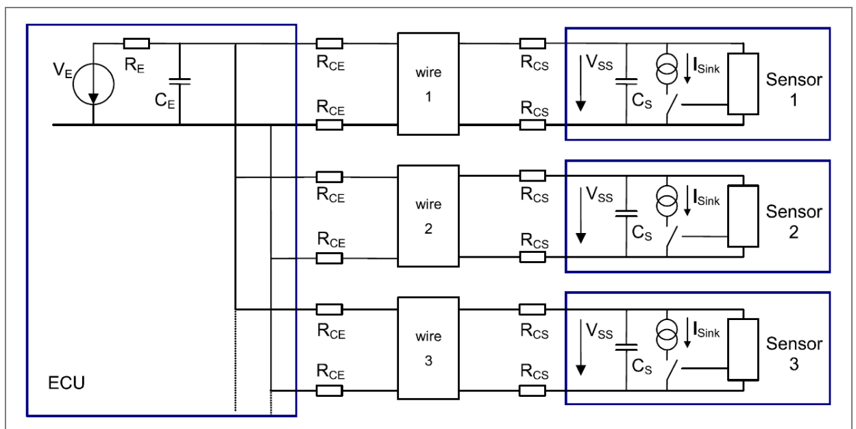
Figure 33: Synchronous parallel bus mode (PSI5-P)
