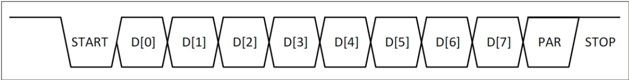
Figure 9: UART protocol frame
