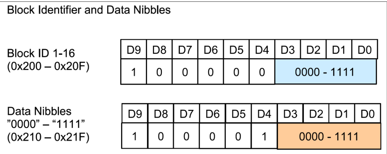
Figure 30: Block ID and data nibbles
