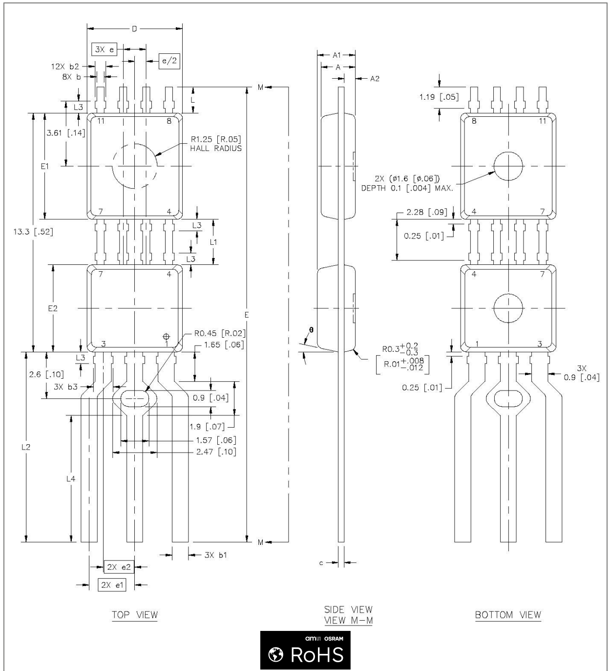
Figure 36: SIP package outline drawing
