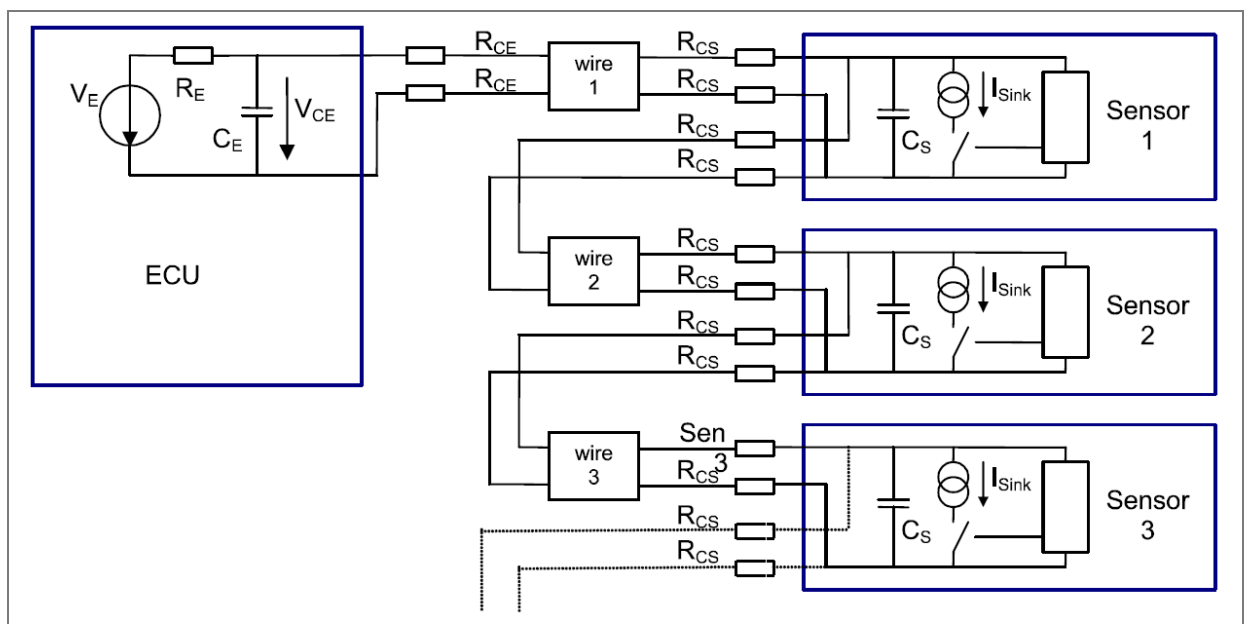
Figure 34: Synchronous parallel bus mode (PSI5-P)
