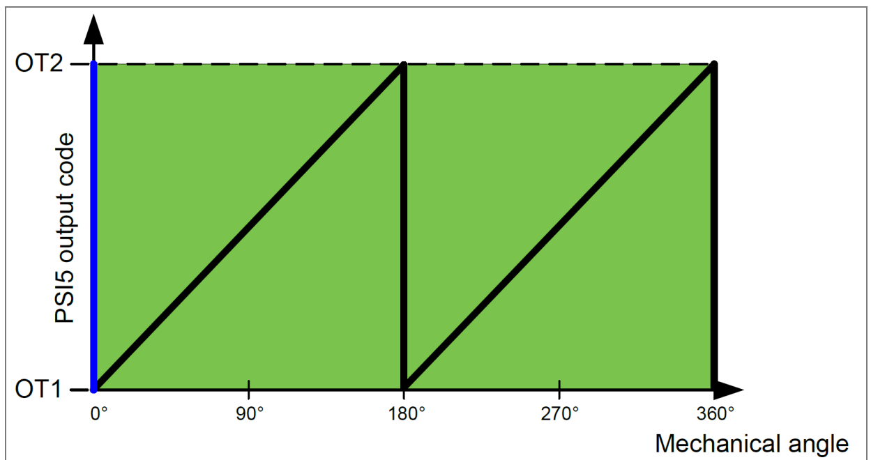
Figure 14: Dual quadrant
