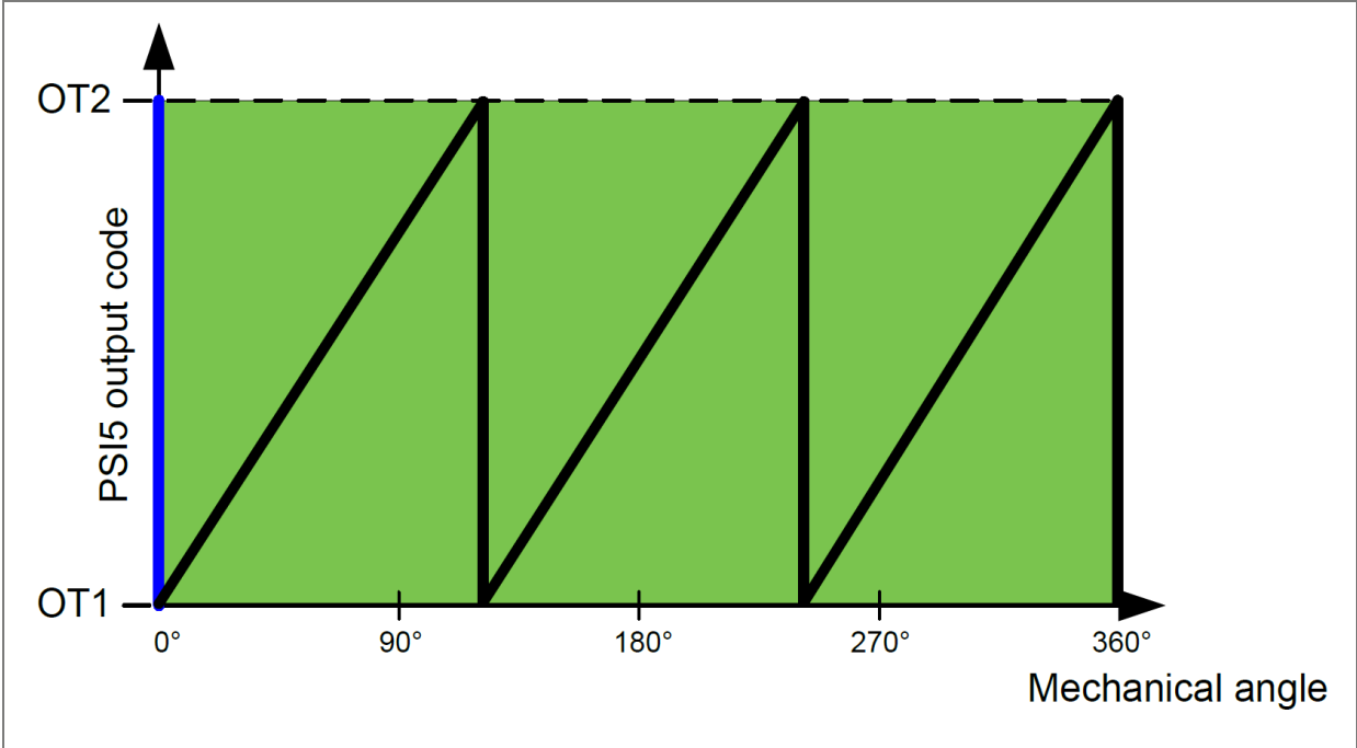
Figure 15: Triple quadrant
