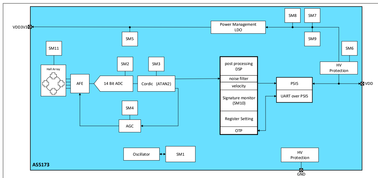
Figure 1: Functional blocks of AS5173
