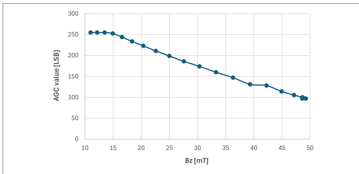
Figure 3: Typical relation between B_z (1) and AGC value
