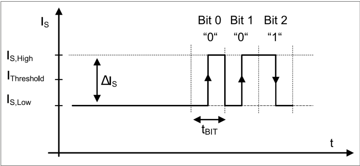
Figure 23: Bit encoding using supply current modulation
