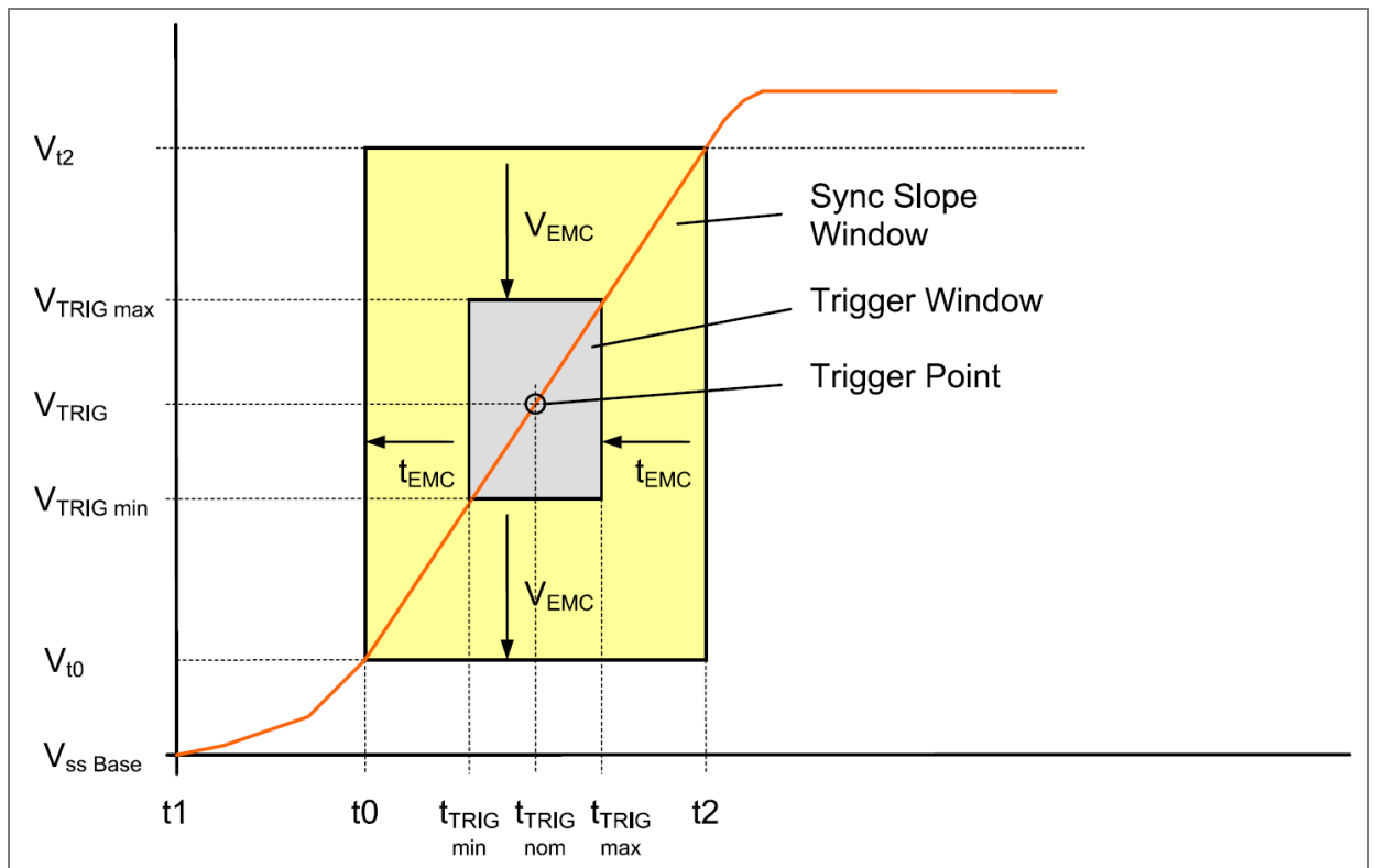
Figure 5: Trigger window
