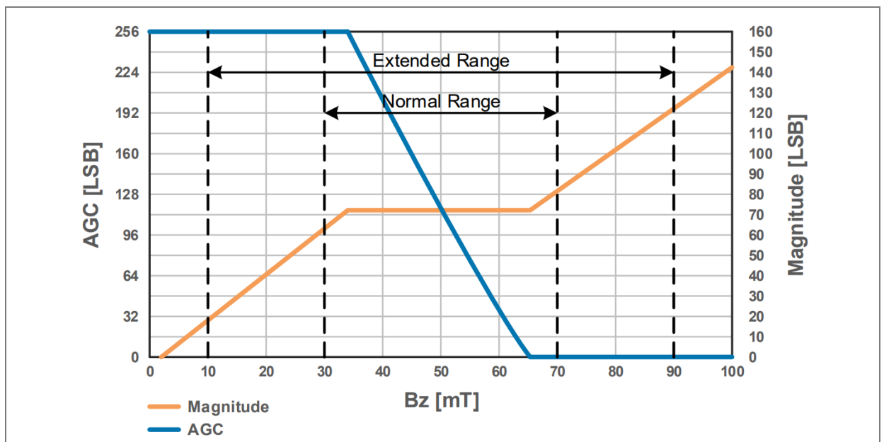
Figure 17: Typical relationship between AGC, magnitude and flux density
