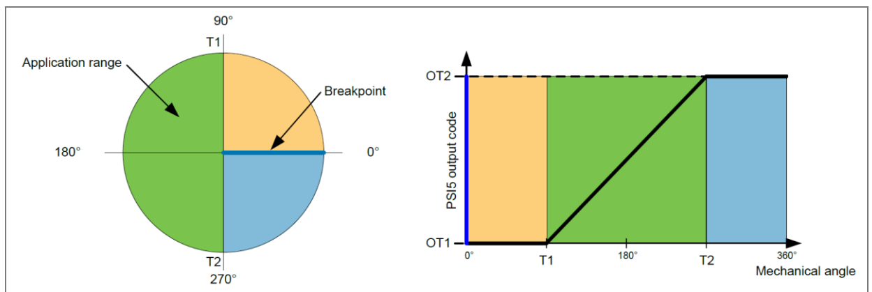
Figure 12: Transfer function
