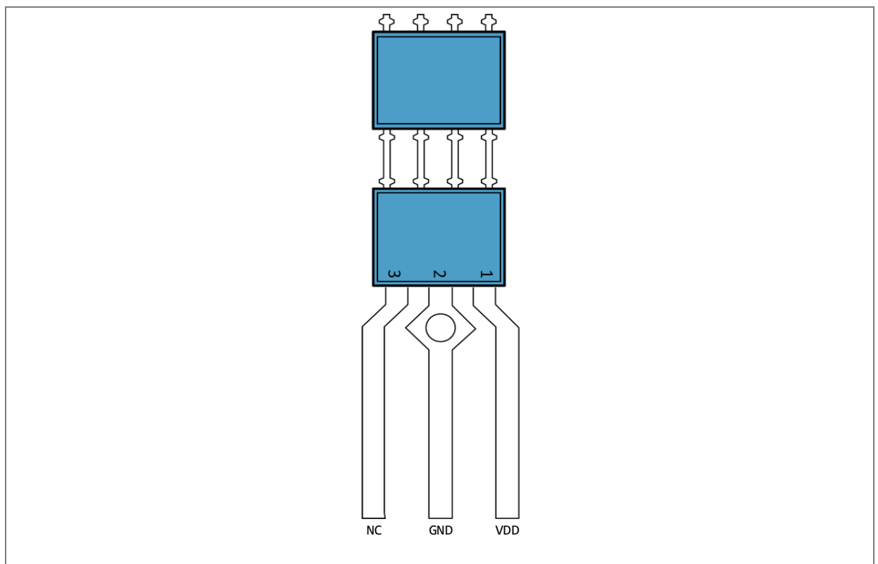
Figure 2: AS5173 package
