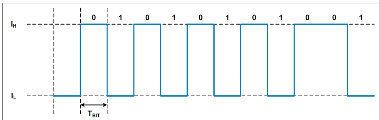
Figure 8: Bit encoding of sensor-to-programmer communication
