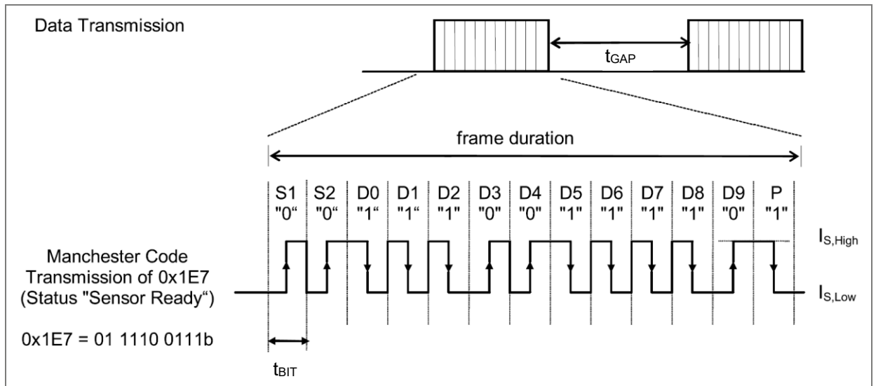
Figure 24: Example of a 10-bit data frame
