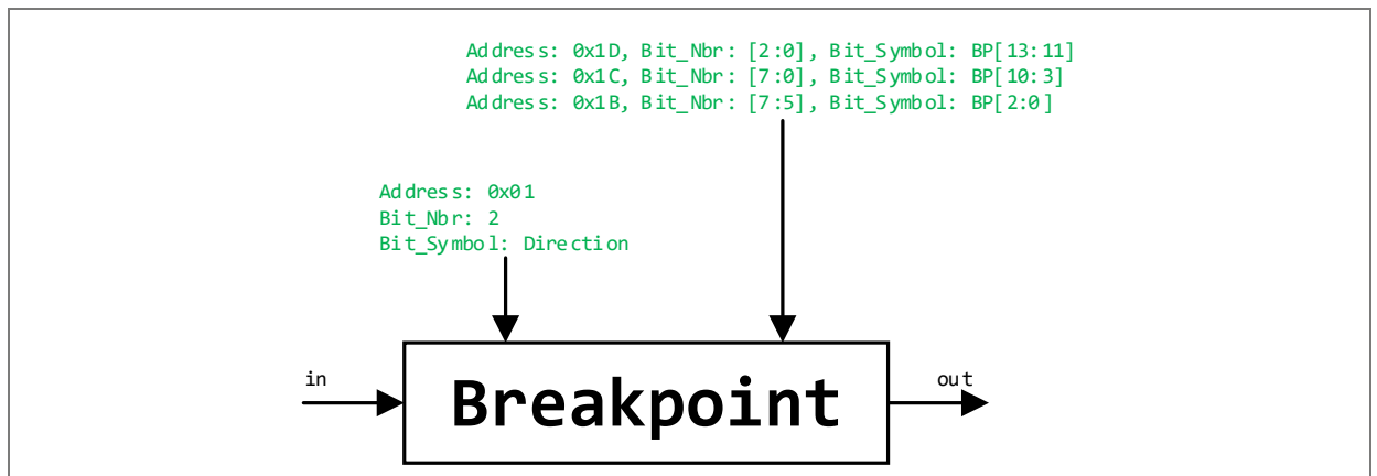
Figure 21: Breakpoint block
