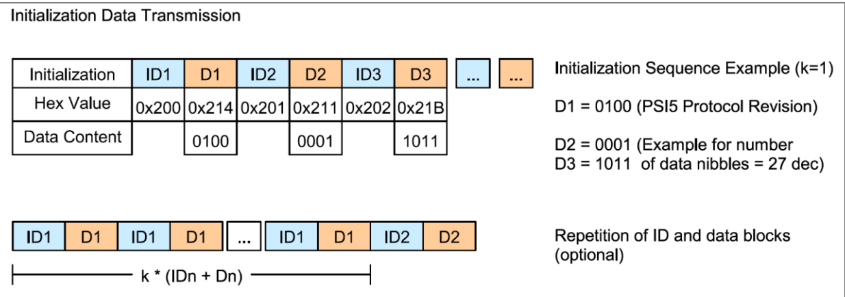
Figure 31: Startup sequence
