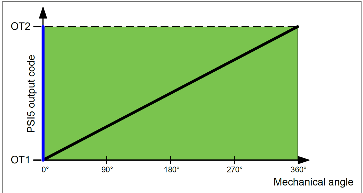
Figure 13: Single quadrant
