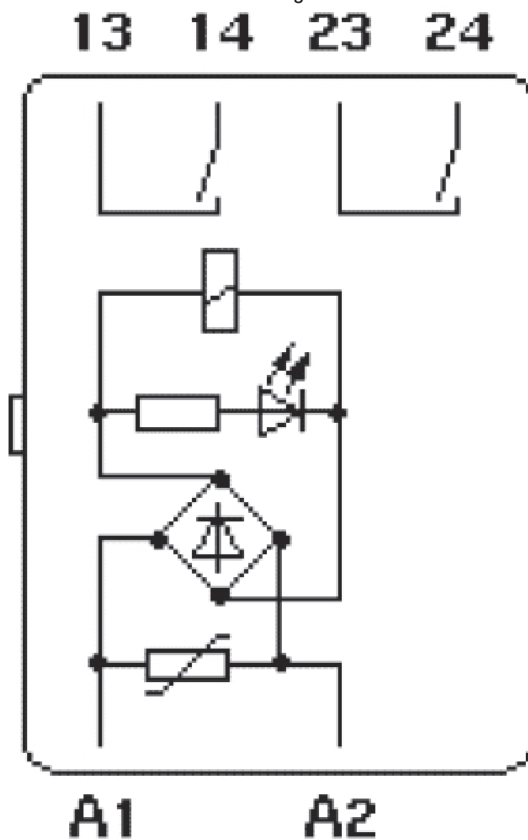
Circuit diagram
