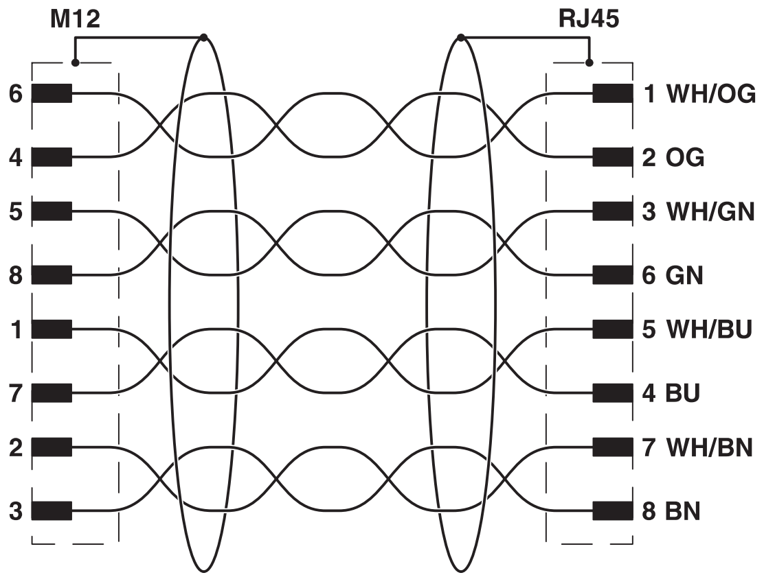
M12和RJ45针式引脚分配
