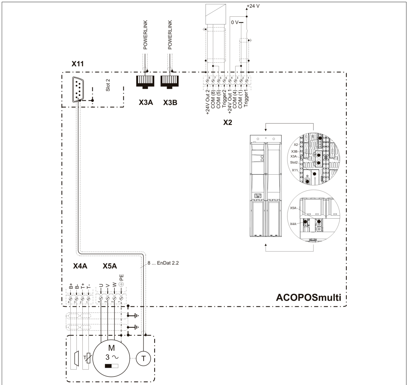
Figure 7: Pinout overview
