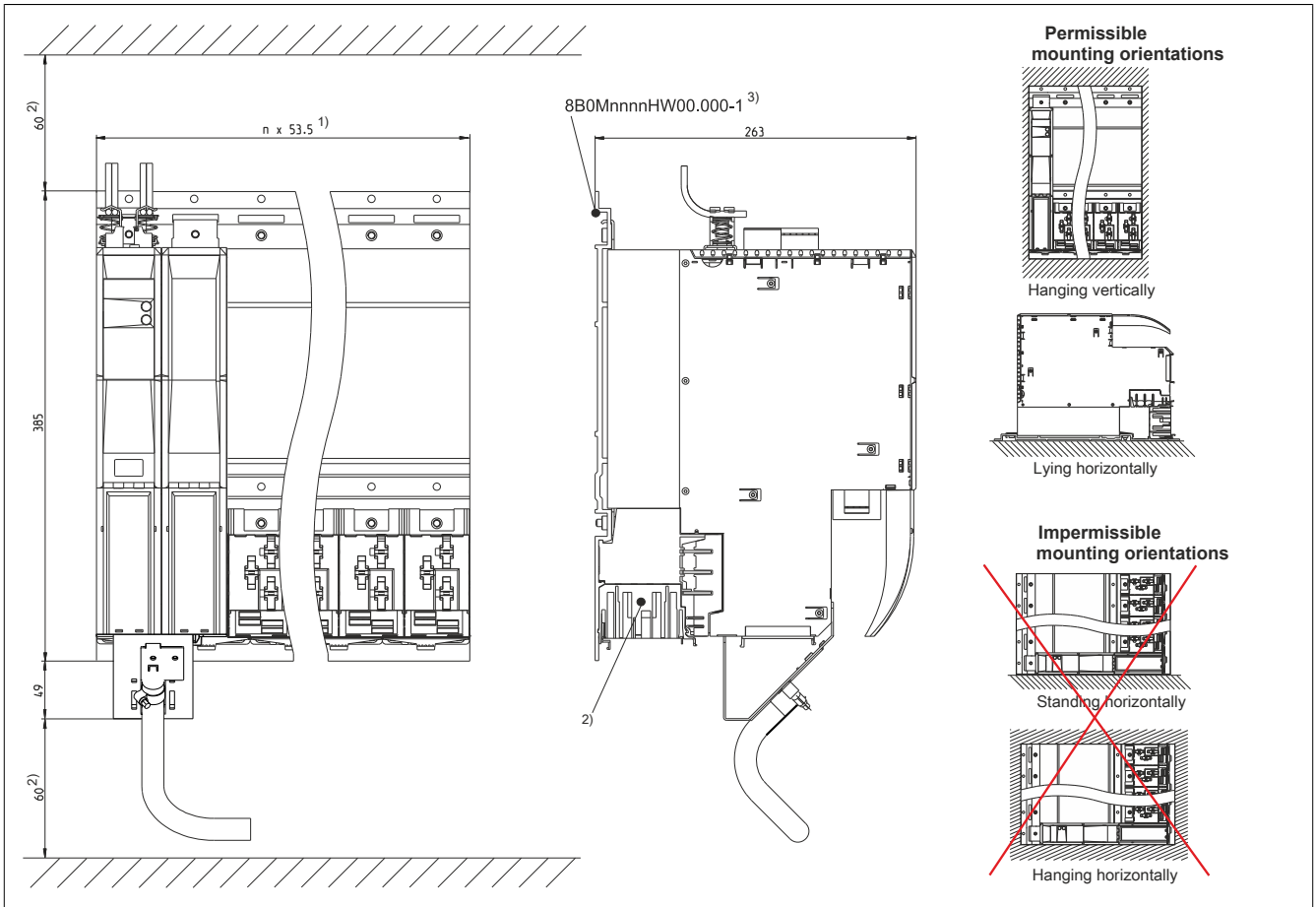
Figure 6: Dimension diagram and installation dimensions
