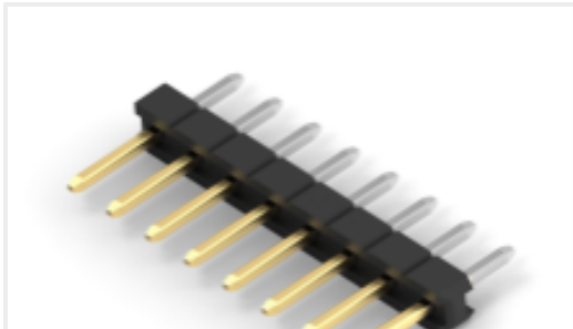
TE Part #2842111-8 8P,2MM,BRK HDR,SRRT,2.8,0.38AU,TB
