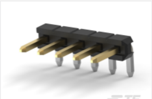
TE Part #2842124-5 5P,2MM,BRK HDR,SRRT,2.8,0.76AU, BOX
