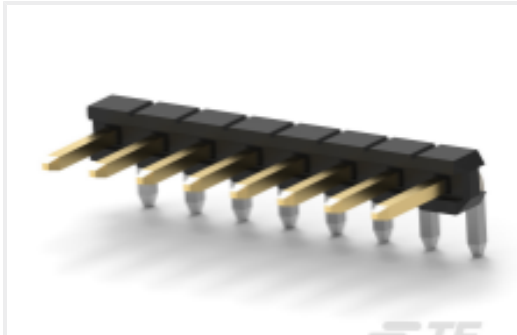
TE Part #2842111-8 8P,2MM,BRK HDR,SRRT,2.8,0.38AU,TB
