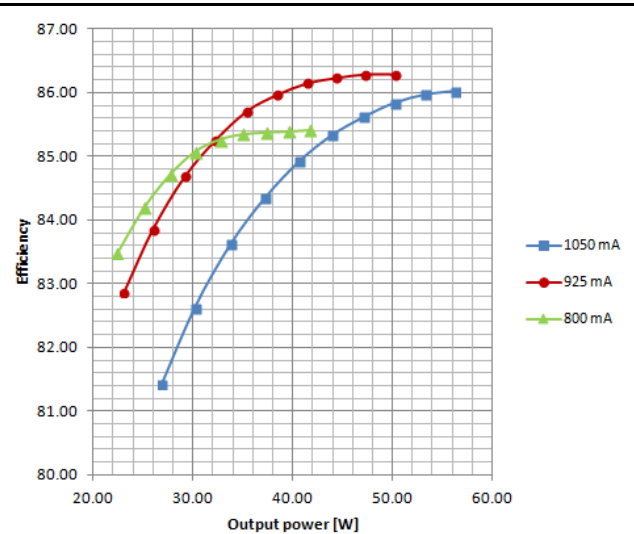
Typical Efficiency over load
