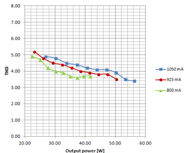
Typical THD over load
