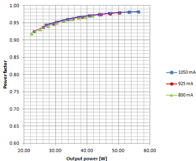
Typical Power factor over load
