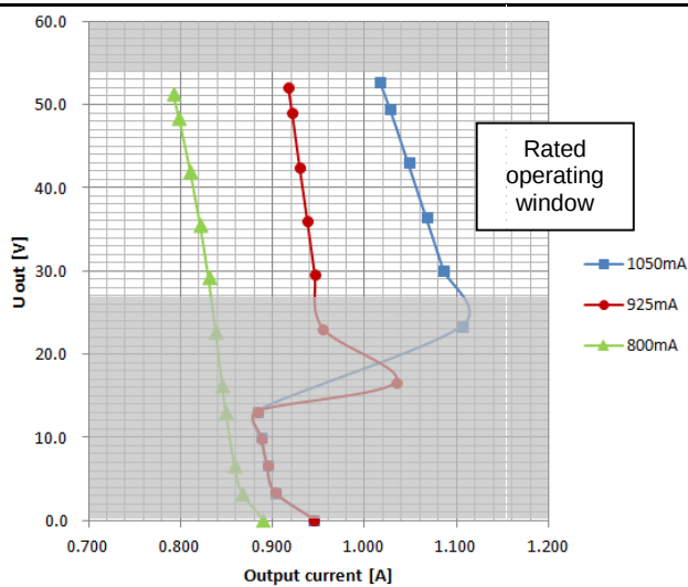
Typical Operating window
