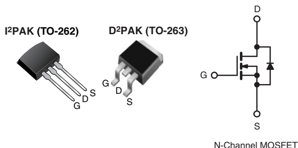
N-Channel MOSFET
